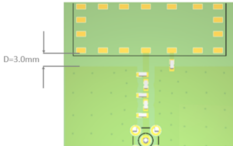
All dimensions in (mm)
