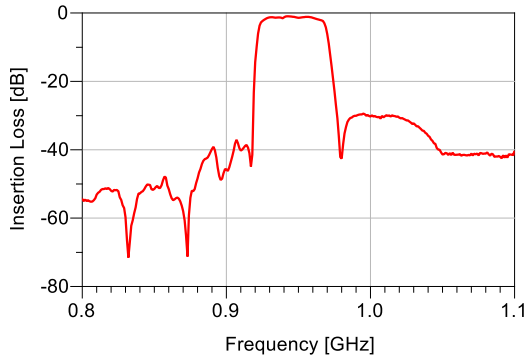
Insertion Loss
