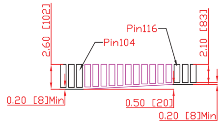
Detail D
