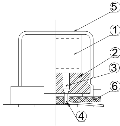
Fig. 1 Cross-section view
