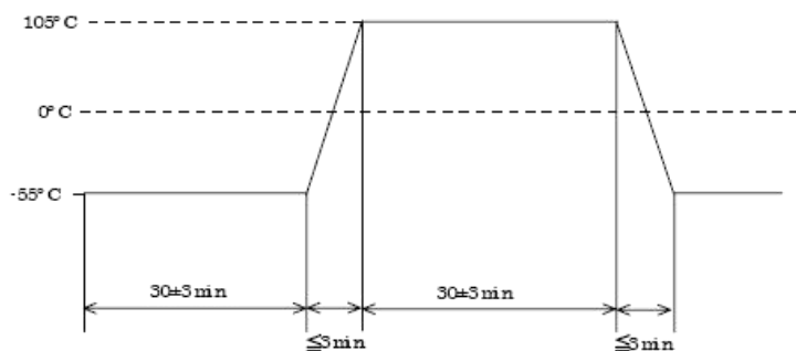
Fig. 5 Rapid temperature change profile
