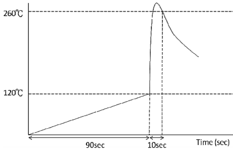
Figure 6 Flow Curve
