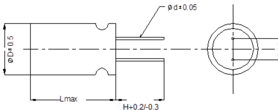
Figure 2 Dimension
