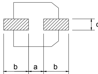
Figure 5 Soldering pad
