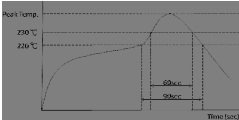
Figure 4 Reflow profile
