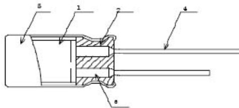
Fig. 1 Cross-section view
