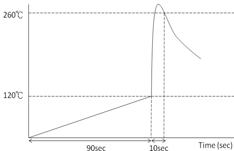
Figure 6 Flow Curve
