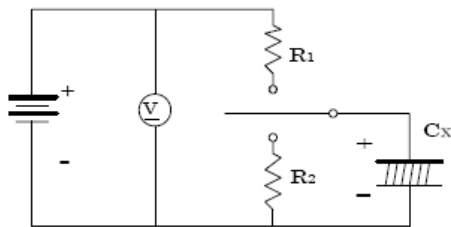
Fig. 4 Surge voltage circuit
