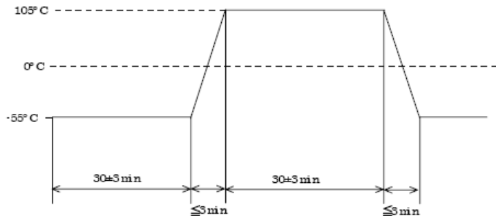
Fig. 5 Rapid temperature change profile
