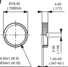
KNURLED NUT
