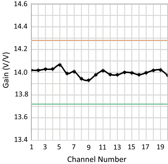
Figure 13: Channel to Channel Gain Variation Five (5) Units
