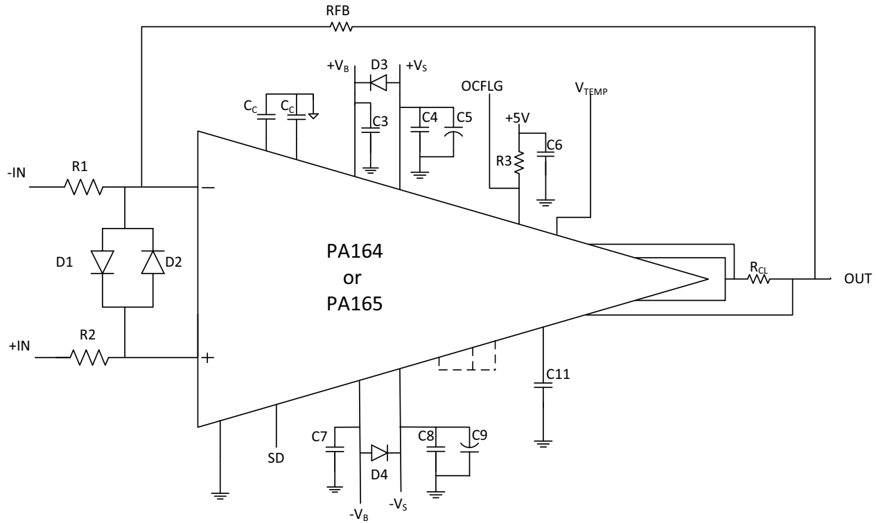
Figure 2: Typical Connection
