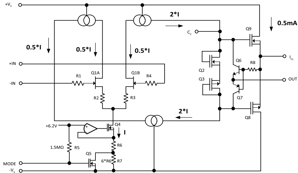
Figure 1: Equivalent Schematic
