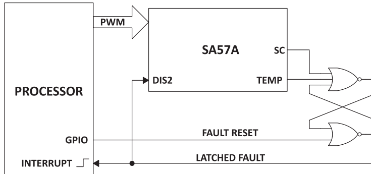
Figure 16: External Fault Latch Circuit
