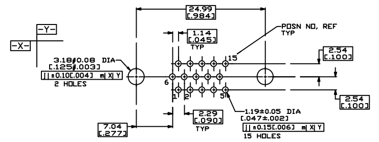
P.C. BOARD MOUNTING DIMENSIONS
