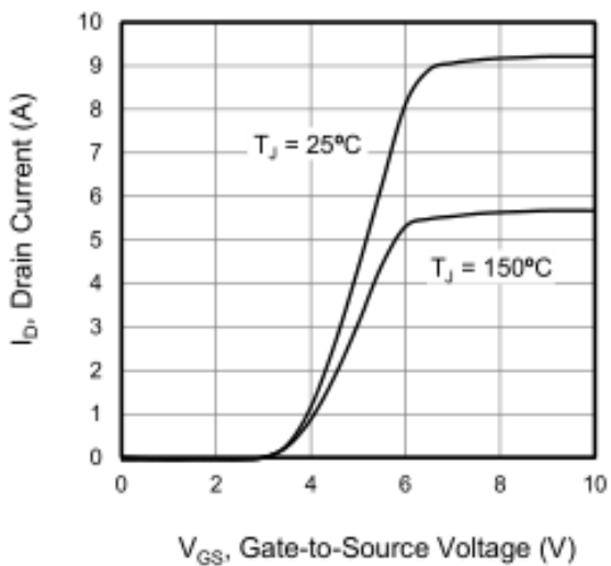
Figure 5. Transfer Characteristics
