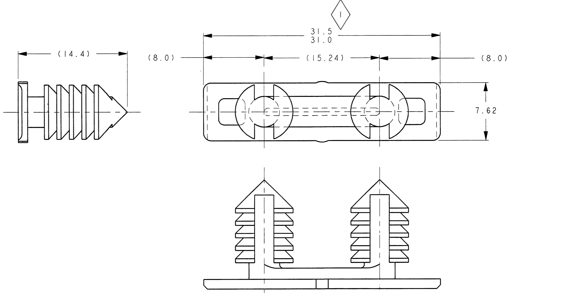
P/N G62000-A SHOWN TYPE "A" UNIVERSAL DESIGN DIMENSIONS SAME AS TYPE "B" EXCEPT AS SHOWN (NOTE: NOT TOOLED AT FCI)
