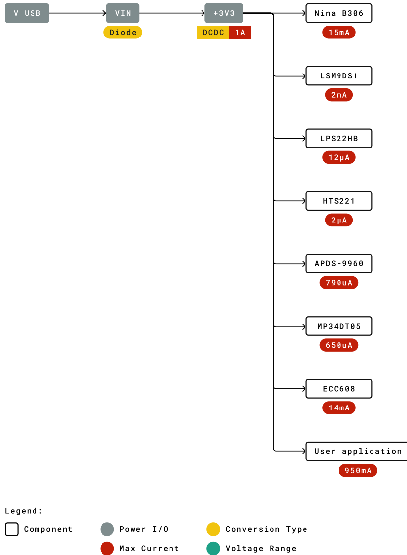
Power tree
