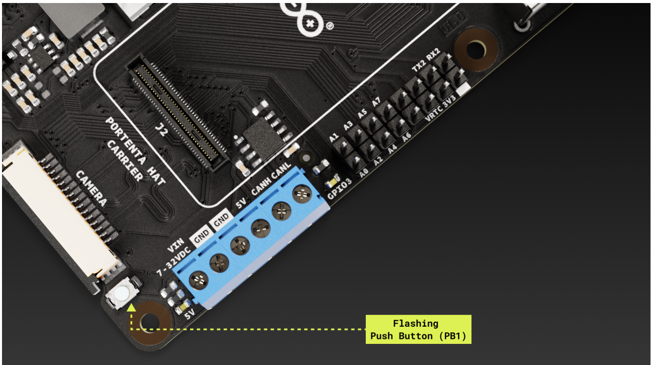
Figure 15. Flashing push button of the Portenta Hat Carrier
