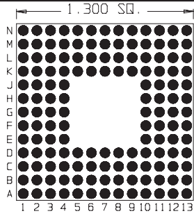
144 Pins Footprint 13003
