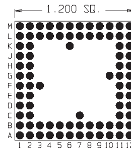
84 Pins Footprint 12011
