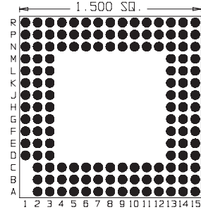
141 Pins Footprint 15029
