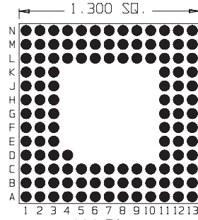
121 Pins Footprint 13013
