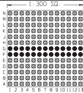
26 Pins Footprint 13087
