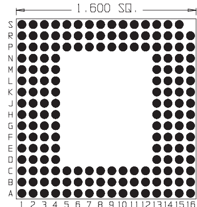
175 Pins Footprint 16008
