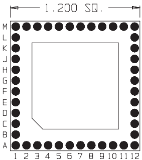
44 Pins Footprint 12019
