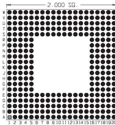
299 Pins Footprint 20015
