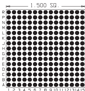
225 Pins Footprint 15001
