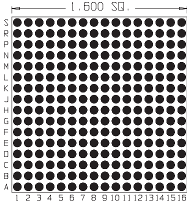
256 Pins Footprint 16001
