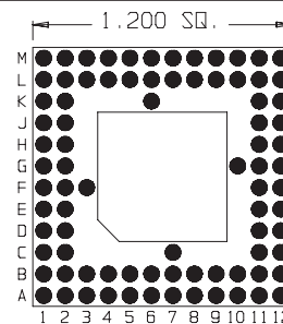
84 Pins Footprint 12010
