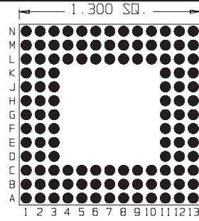
120 Pins Footprint 13015
