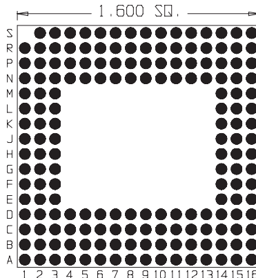
175 Pins Footprint 16005
