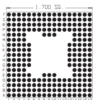
225 Pins Footprint 17008
