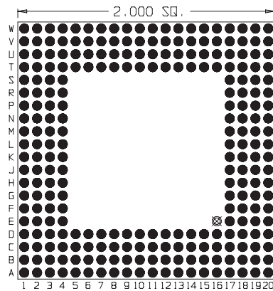
256 Pins Footprint 20017
