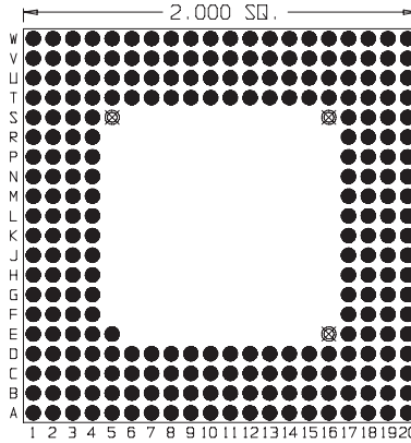
257 Pins Footprint 20013
