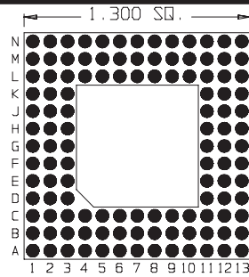
120 Pins Footprint 13014
