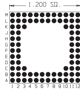
84 Pins Footprint 12013
