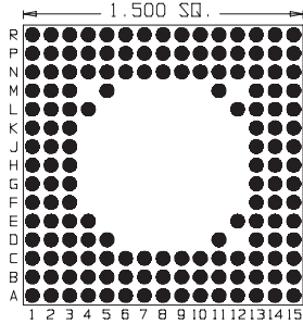
153 Pins Footprint 15017
