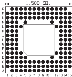
149 Pins Footprint 15018
