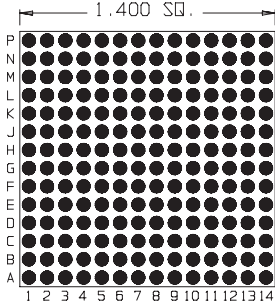
196 Pins Footprint 14001
