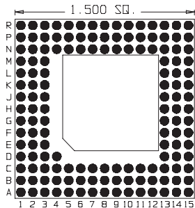
145 Pins Footprint 15023
