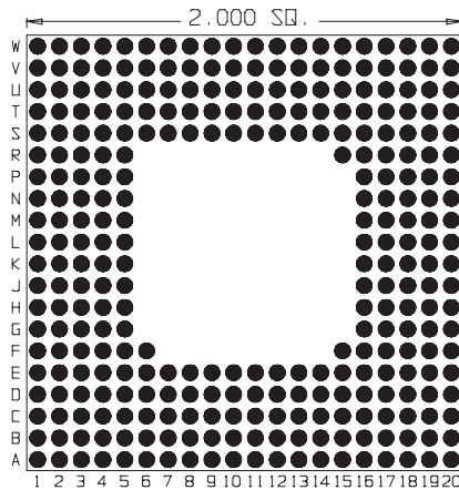
303 Pins Footprint 20004
