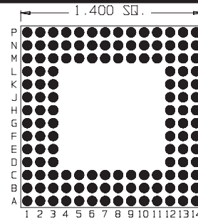
132 Pins Footprint 14016
