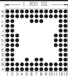
100 Pins Footprint 13082
