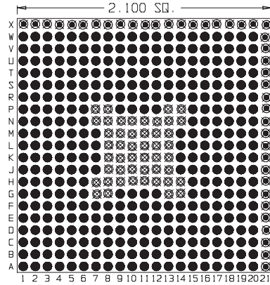
352 Pins (393) Footprint 20016
