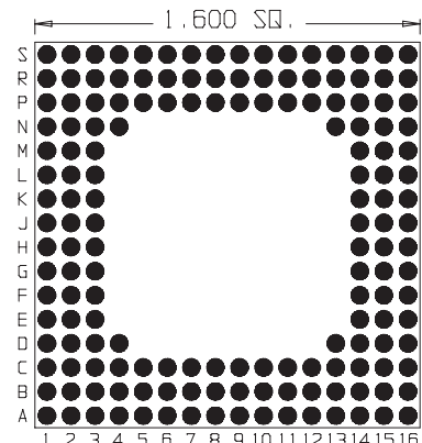
159 Pins Footprint 16009
