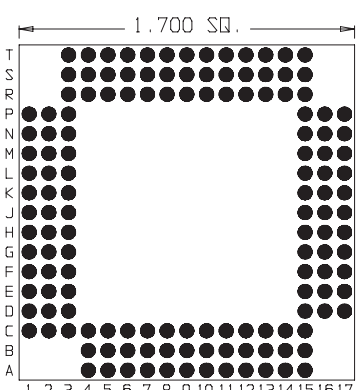
144 Pins Footprint 17006
