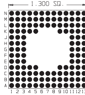
128 Pins Footprint 13093
