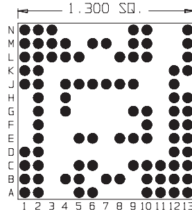
90 Pins Footprint 13089
