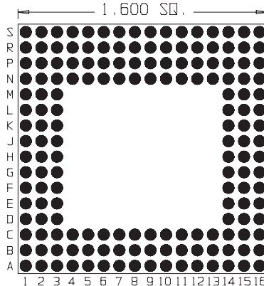
166 Pins Footprint 16004
