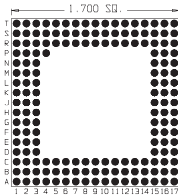
169 Pins Footprint 17002
