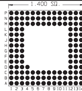
133 Pins Footprint 14014
