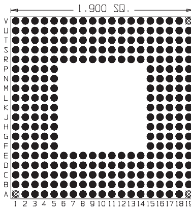
277 Pins Footprint 19005
