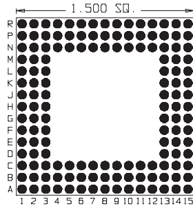
144 Pins Footprint 15026
