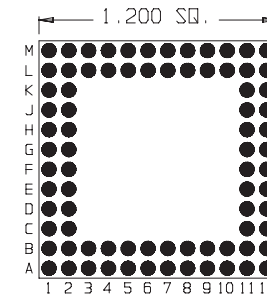
80 Pins Footprint 12015
