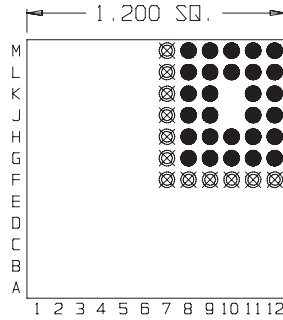
28 Pins Footprint 12021
