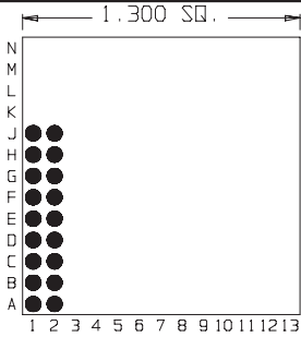
18 Pins Footprint 13083
