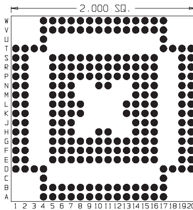
240 Pins Footprint 20014
