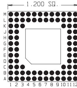
84 Pins Footprint 12012
