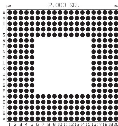
300 Pins Footprint 20006
