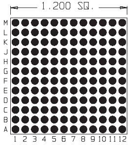
144 Pins Footprint 12001
