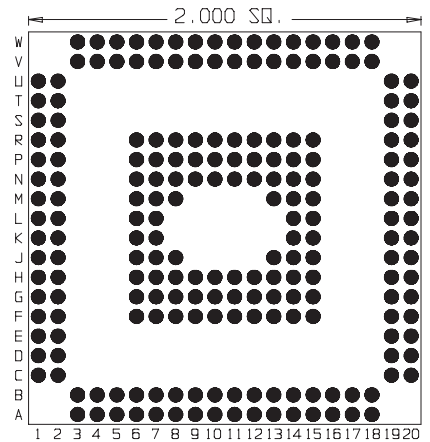
208 Pins Footprint 20008
