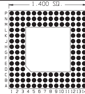
132 Pins Footprint 14015
