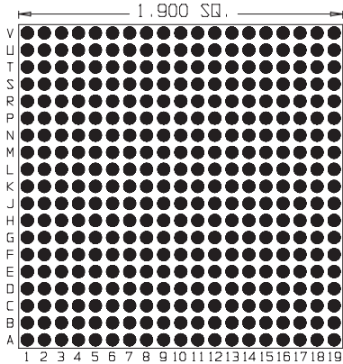
361 Pins Footprint 19001
