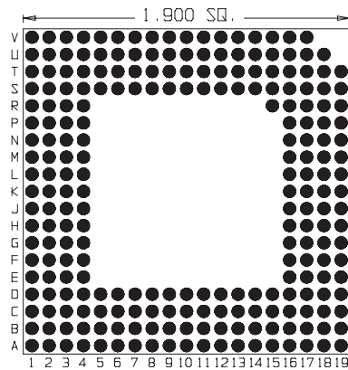
238 Pins Footprint 19007
