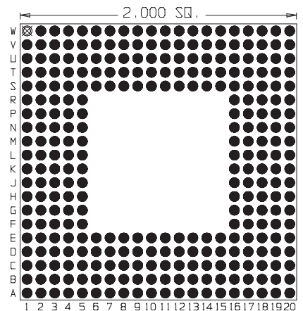
299 Pins Footprint 20009
