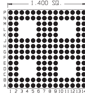
160 Pins Footprint 14009
