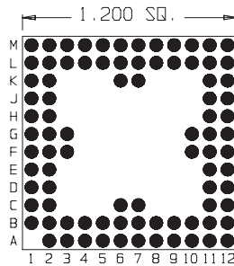
88 Pins Footprint 12009
