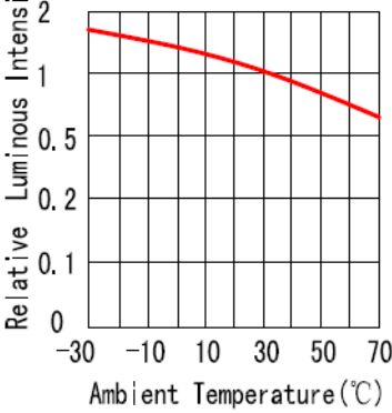
LUMINOUS INTENSITY VS. AMBIENT TEMPERATURE
