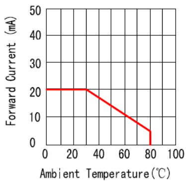
ALLOWABLE FORWARD CURRENT AMBIENT TEMPERATURE
