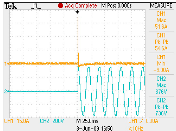
Figure 6: ADNB034-12-1PM-C Inrush Current Vin = 264Vac Load: Io = 3.4A Ta = 25 °C Ch 1: Iin Ch 2: AC Mains
