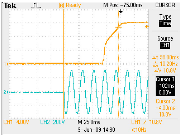
Figure 3: ADNB034-12-1PM-C Turn-on delay – Vin= 90Vac Load: Io = 3.4A Ta = 25 °C Ch 1: Vo Ch2:AC Mains
