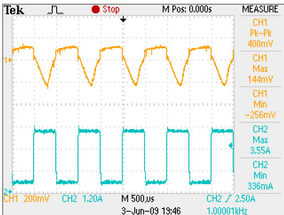
Figure 5: ADNB034-12-1PM-C Transient Response Vin = 230Vac Load: Io = FULL/MIN LOAD, 90%DUTY/1KHZ Ch 1: Vo Ch 2: Iout
