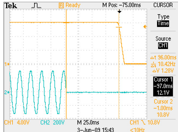
Figure 4: ADNB034-12-1PM-C Hold Up Time –Vin=90Vac Load: Io = 3.4A Ta = 25 °C Ch 1: Vo Ch 2: AC Mains
