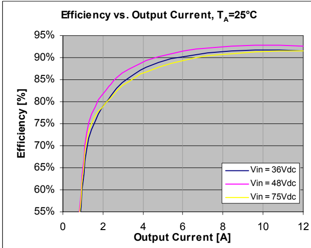
Figure 13. Efficiency vs. Load Current at I_O = \text{Full Load} , T_A = 25^\circ\text{C} (ambient temperature).
