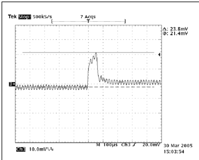
Figure 41. Transient Response at T_A = 25^\circ\text{C} , 1.8V_{\text{OUT}} Deviation (Hi-Lo).
