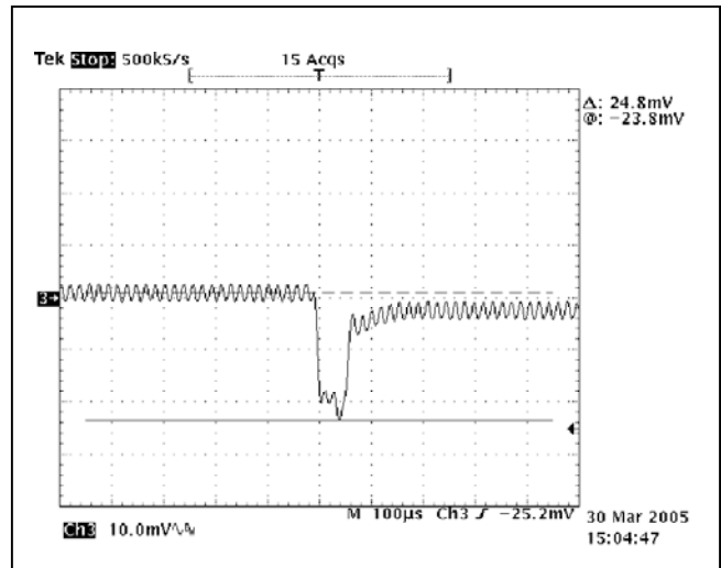
Figure 42. Transient Response at T_A = 25^\circ\text{C} , 1.8V_{\text{OUT}} Deviation (Lo-Hi).
