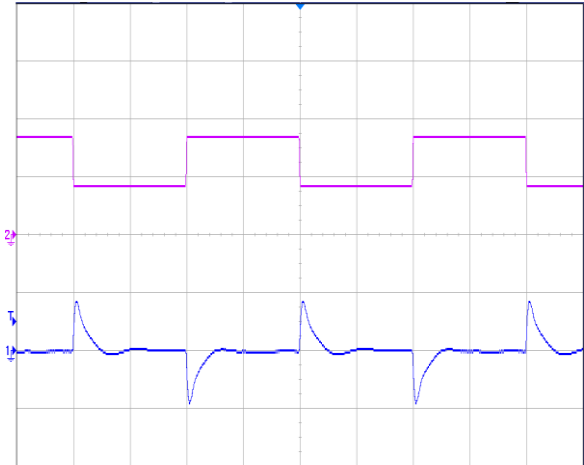
Figure 4 Dynamic response for 25% load step (25% ~ 50% ~ 25%) and 0.1A/ \mu s slew rate, see Figure 11 for test configuration, CH1-output voltage (500mV/div); CH2-output current (5A/div)
