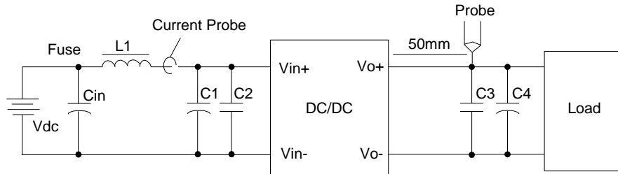
Figure 16 Ripple & noise test configuration
