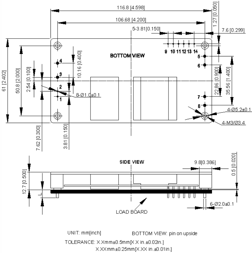
Figure 18 Mechanical diagram
