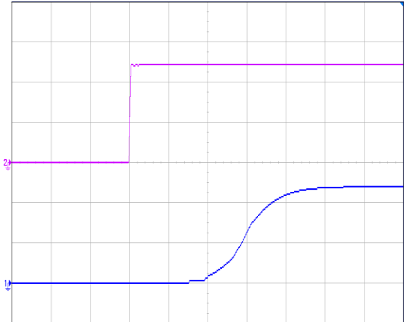
Figure 6 Output voltage startup by power on, (100ms/div), see Figure 11 for test configuration, CH2-input voltage (20V/div); CH1-output voltage (20V/div)
