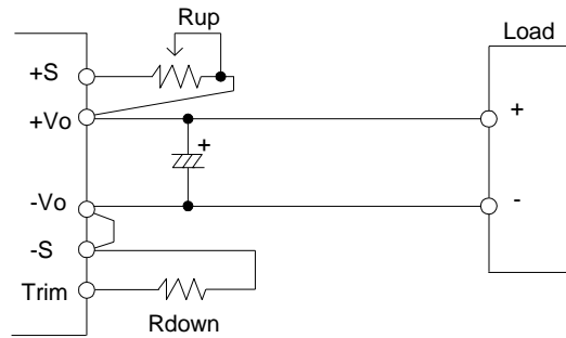
Figure 14 Trim circuit
