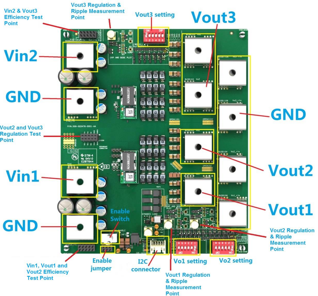
Fig. 2 – LGA80D setup
