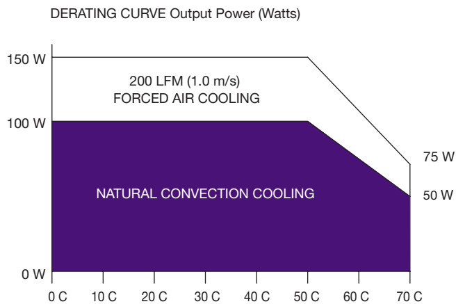
Figure 1: Derating Curve
