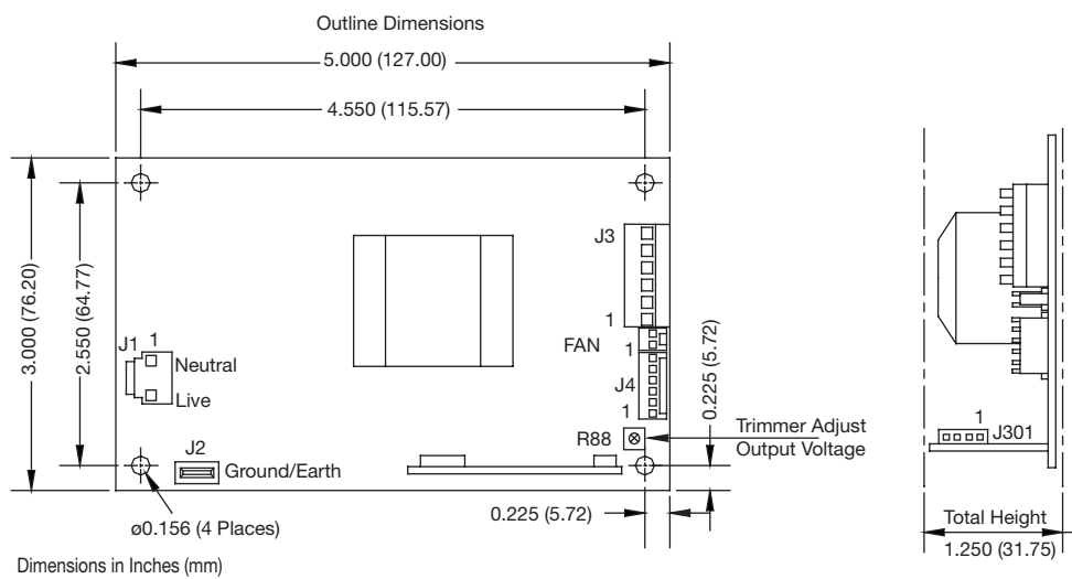
Figure 2: Mechanical Drawing
