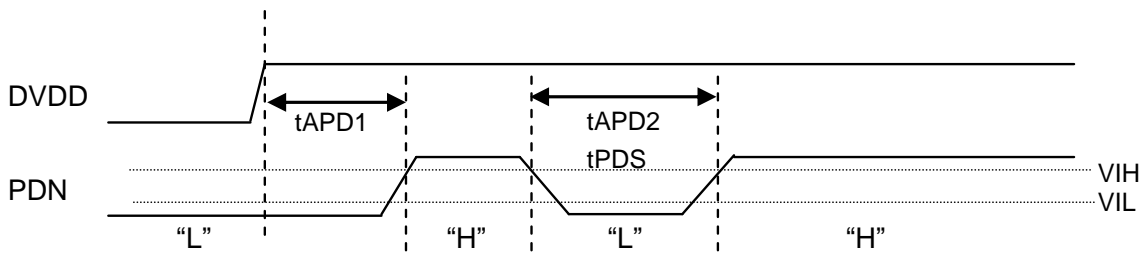
Figure 15. PDN
