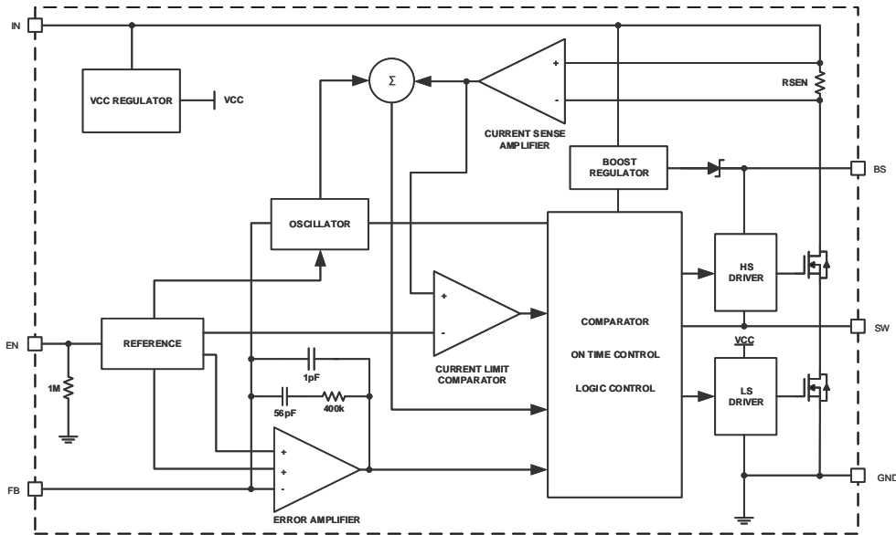
Figure 2. ASP8120 Block Diagram
