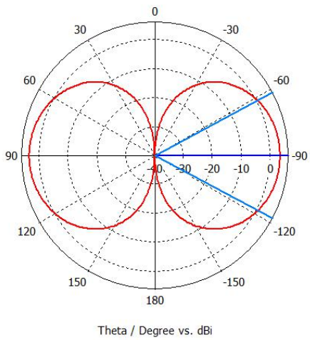
Farfield (Array) Directivity Abs (Phi=90)
