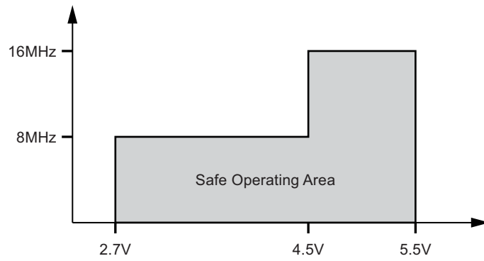
Figure 2-1. Maximum Frequency versus V_{CC}
