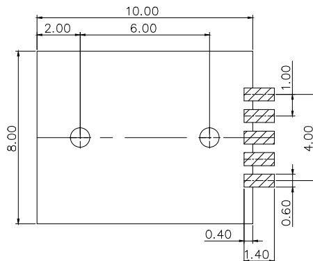
PCB LAYOUT TOLERANCE:±0.1 LAND METAL MASK t=0.12
