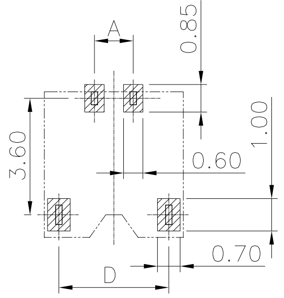
RECOMMENDED P.C BOARD LAYOUT (TOP VIEW) TOLERANCES UNLESS OTHERWISE SPECIFIED ±0.05
