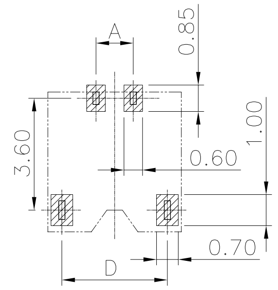
RECOMMENDED P.C BOARD LAYOUT (TOP VIEW) TOLERANCES UNLESS OTHERWISE SPEC+/-0.05 ▨ PAD AREA
