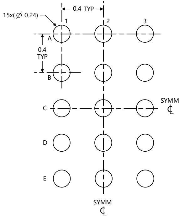
LAND PATTERN EXAMPLE EXPOSED METAL SHOWN SCALE: X40
