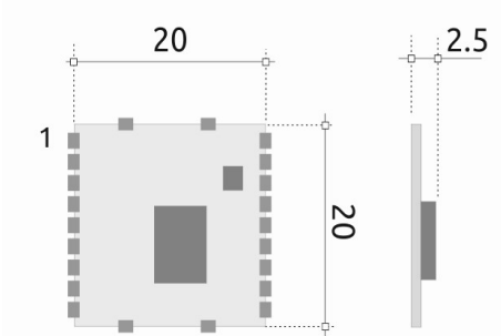
Figure 1: Pin-out and mechanical drawing
