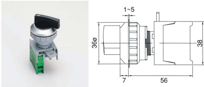
LSS30-1O/C , 1-2
