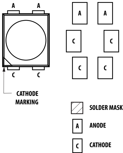
Figure 14. Recommended Soldering Pad Pattern
