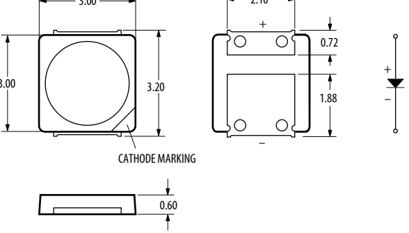
ASMF-LWG4-NxxxD
