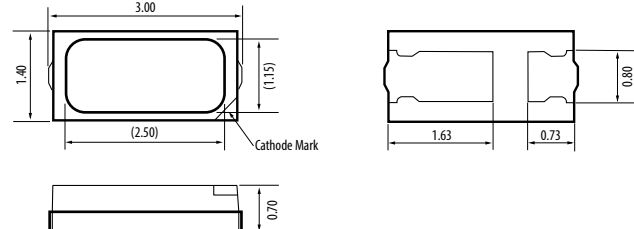
ASMD-LWG3/FWG3 -Nxxxx
