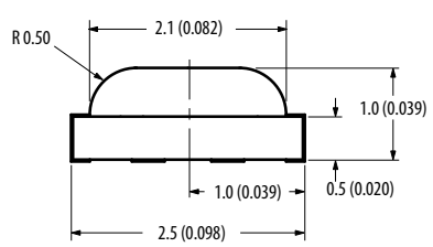
HSMF-C113/C115
