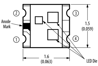
HSMF-C114
