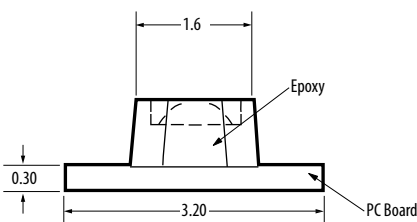
HSMx-C350
