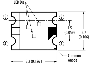
HSMF-C118
