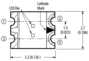
HSMF-C15x
