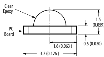
HSMx-C110
