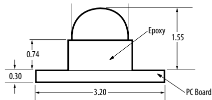
HSMx-C380
