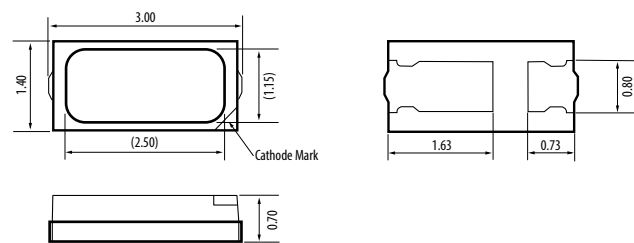
ASMD-LWG3/FWG3 -Nxxxx
