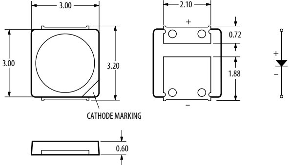
ASMF-LWG4-NxxxD
