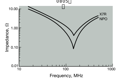
Variation of Impedance with Ceramic Formu Impedance vs. Frequency 1000 pF - COG (NP0) vs X7R 0805
