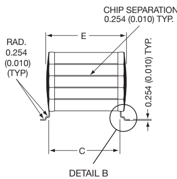
“Z” STYLE LEADS
