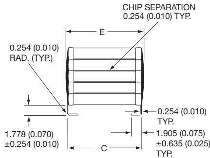
“J” STYLE LEADS
