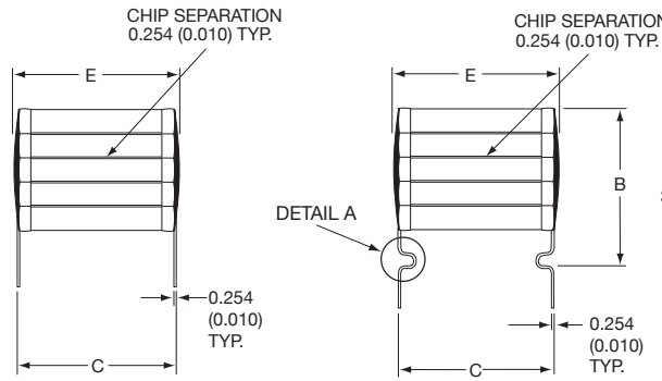
“N” STYLE LEADS
