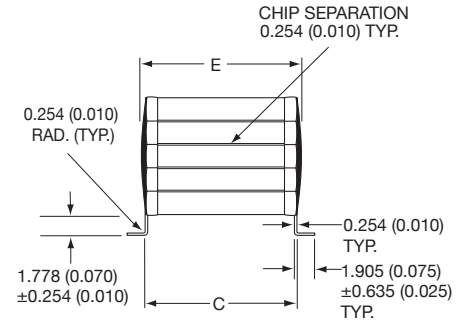
“L” STYLE LEADS
