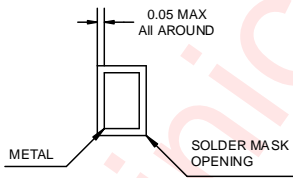
NON-SOLDER MASK DEFINED
