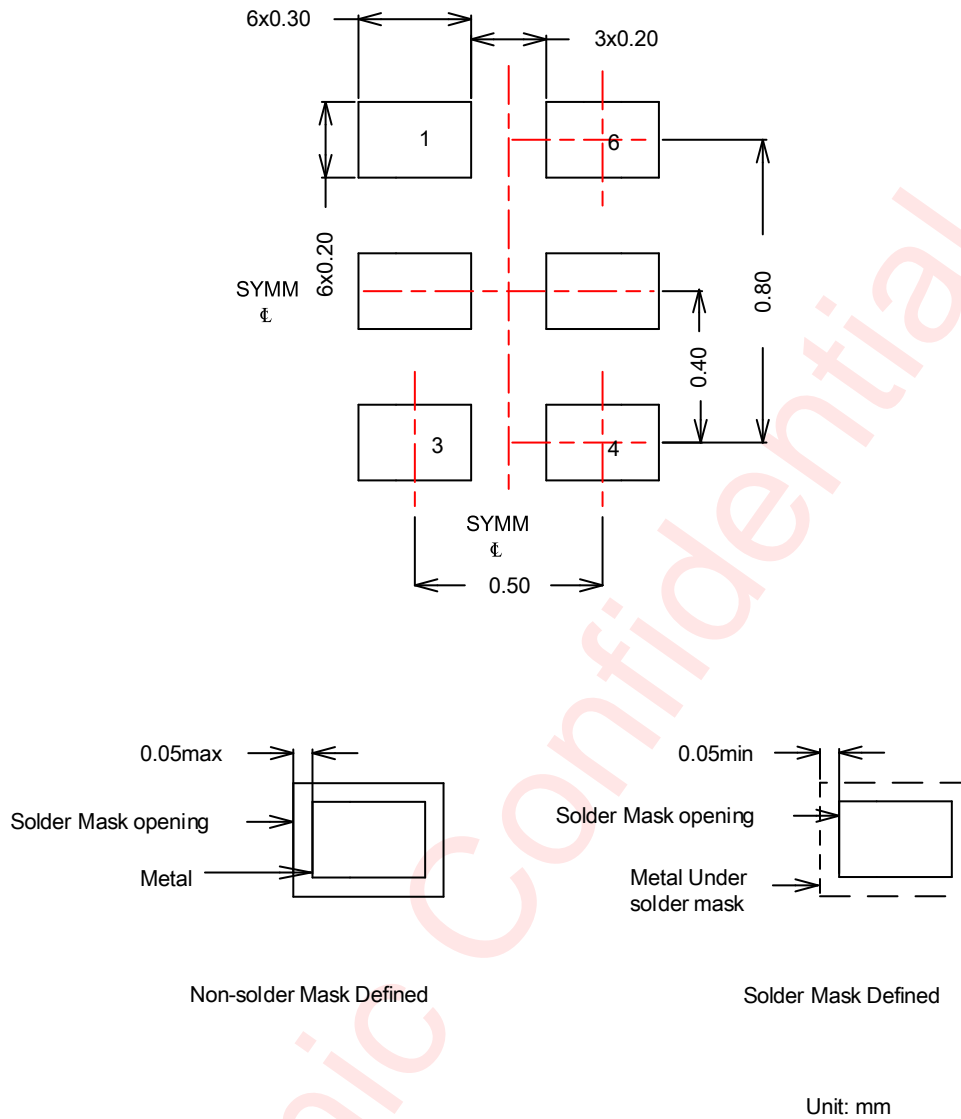
Figure 9 Land Pattern
