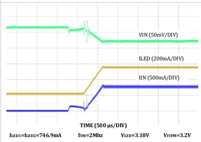
Fig 43. IVFM - Down
