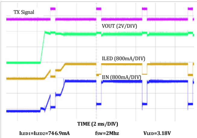
Fig 41. TX Interrupt
