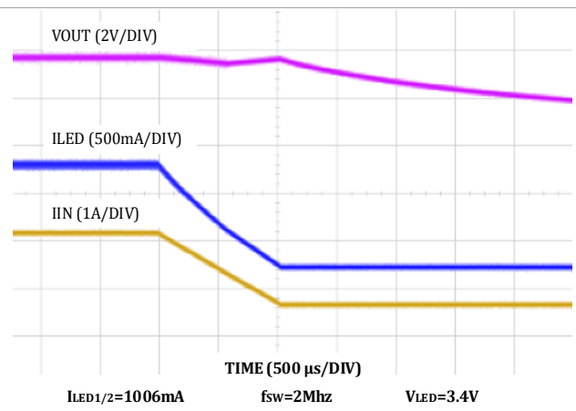
Fig 40. Ramp Down
