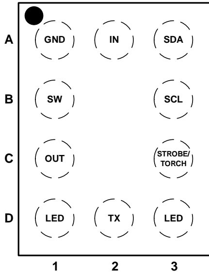
AW36518FCR Pin Configuration (Top View)
