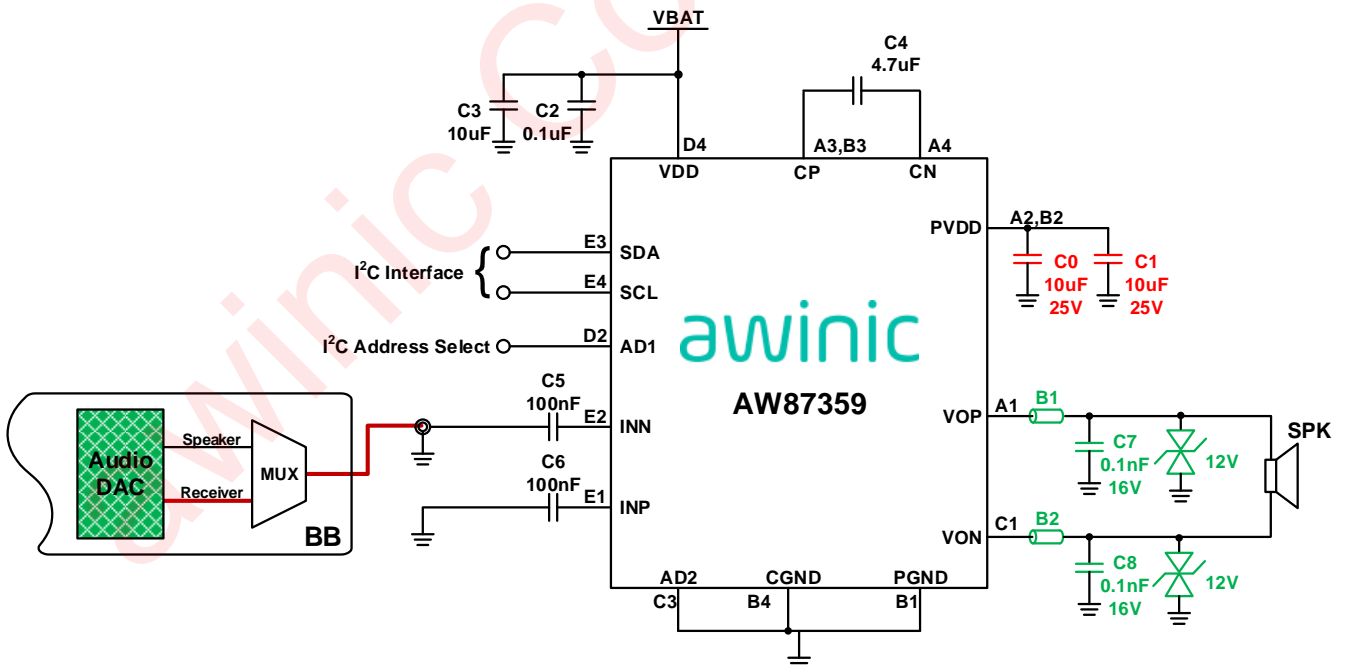
Figure 5 AW87359 Speaker & Receiver 2-in-1 Mode Application Diagram
