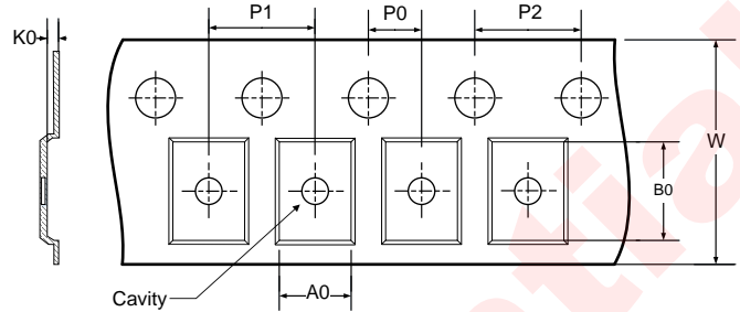
TAPE DIMENSIONS
