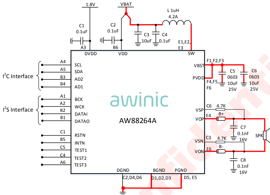
Figure 3 AW88264A Application Circuit
