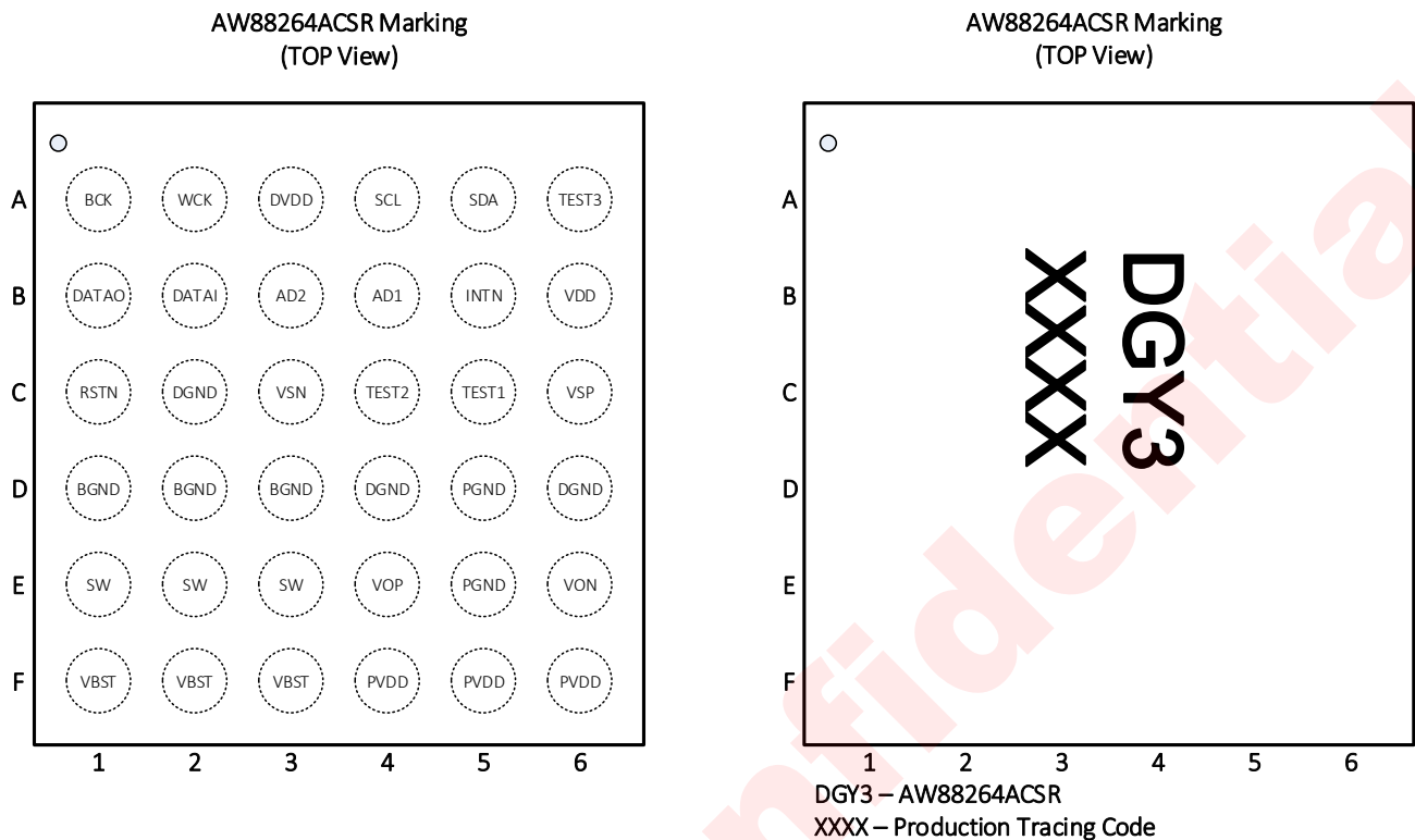
Figure 1 AW88264ACSR pin diagram top view and device marking
