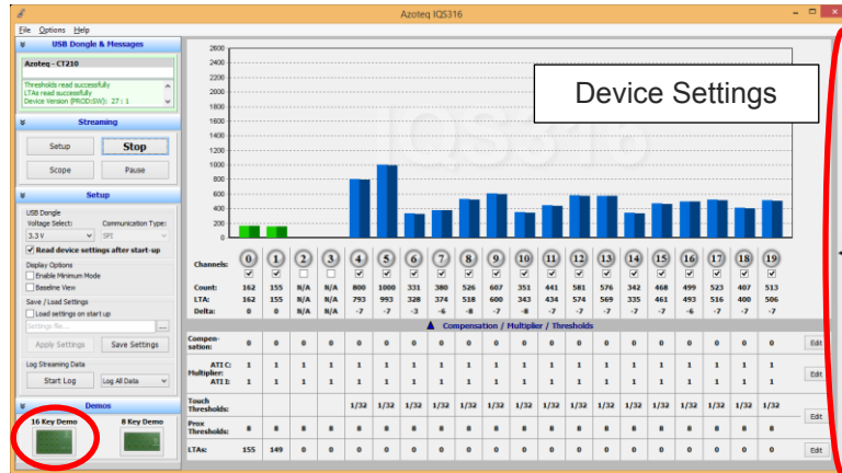
Figure 5.2 Start-up Screen for the IQS316 GUI
