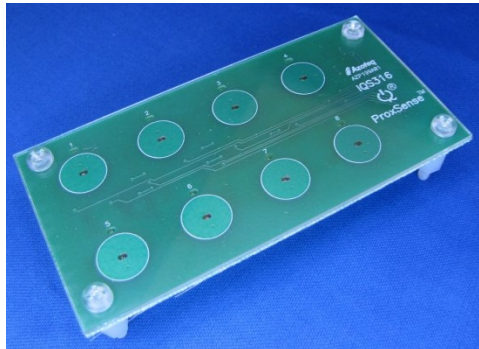
Figure 4.1 8-Key Touch panel
