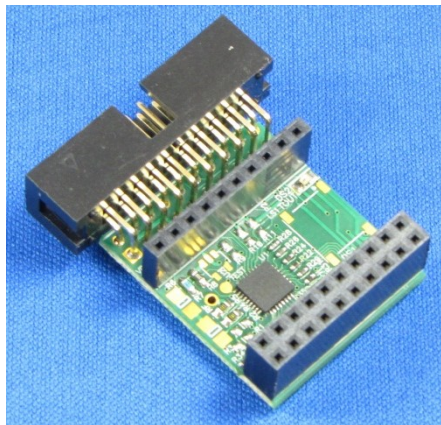
Figure 2.1 Top view of IQS316 EV-Kit controller board
