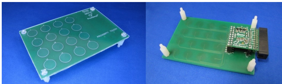
Figure 3.1 16-Key Touch panel (left), 16-Key Touch panel with controller board attached (right)
