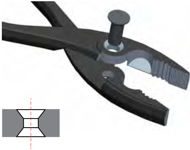
Rivet joints are effective joints for pliers where precision is not a priority.
