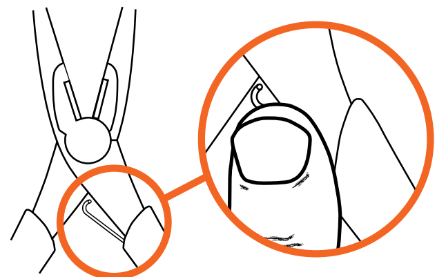
The on-off return spring increases ease of cutting with an automatic opening of the jaws and handles when the grip is loosened.
